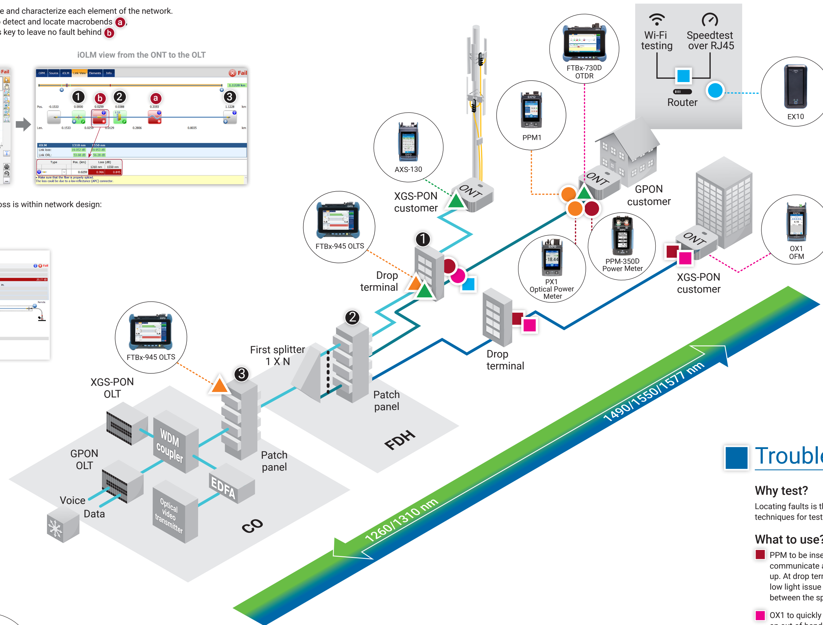
Example of a next generation PON network using GPON, RF video and XGS-PON overlay.
