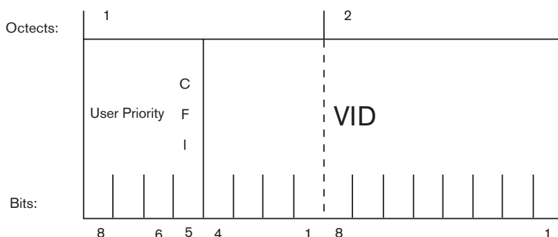
Figure 2: VLAN tag in Ethernet frame
