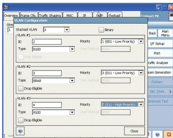
Figure 4: Q-in-Q feature on Packet Blazer
