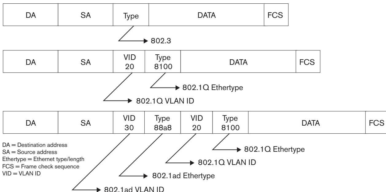
Figure 3: Ethernet, 802.1Q and 802.1ad frames
