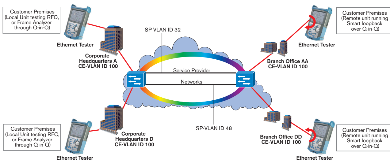
Figure 1: Q in Q example (802.1ad)
