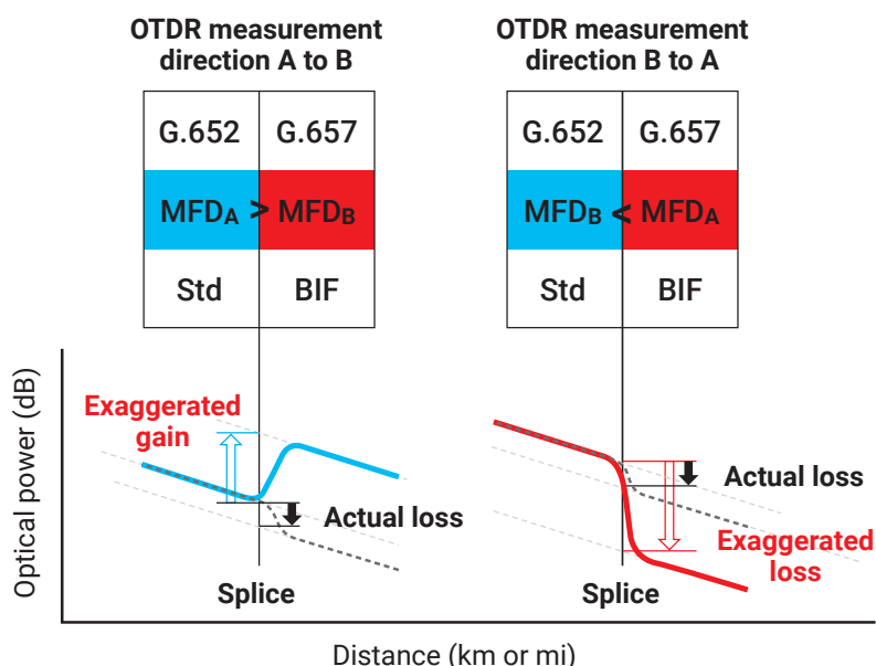
Figure 4. Exaggerated gain and loss due to MFD discontinuity (Courtesy of Corning)
