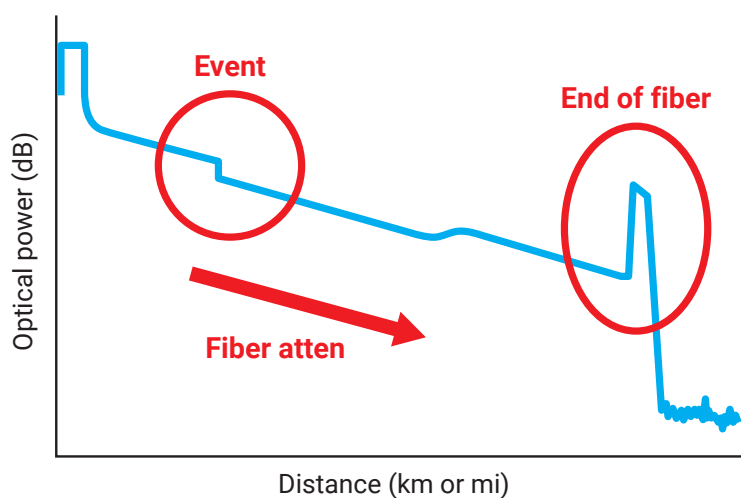
Figure 2. OTDR event examples
