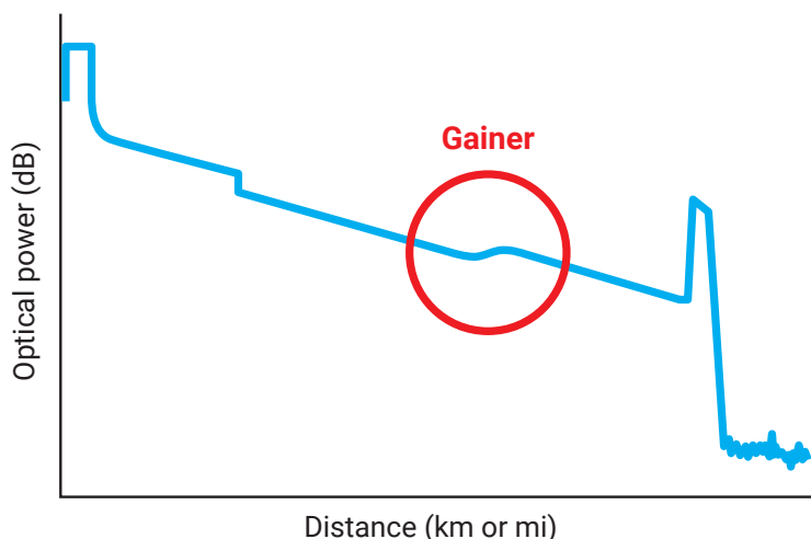
Figure 1. Gainer on simplified OTDR trace
