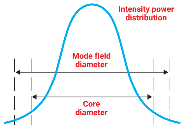
Figure 3. Mode field diameter concept
