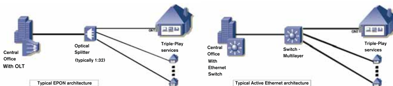
Figure 1: Architecture comparison between active Ethernet and EPON
